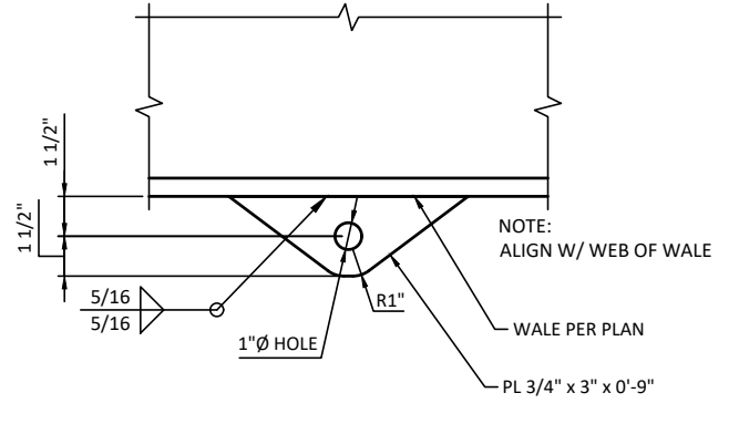
D DETAIL - STAY CHAIN PADEYE FIG 1 SCALE: 3" = 1'-0"
