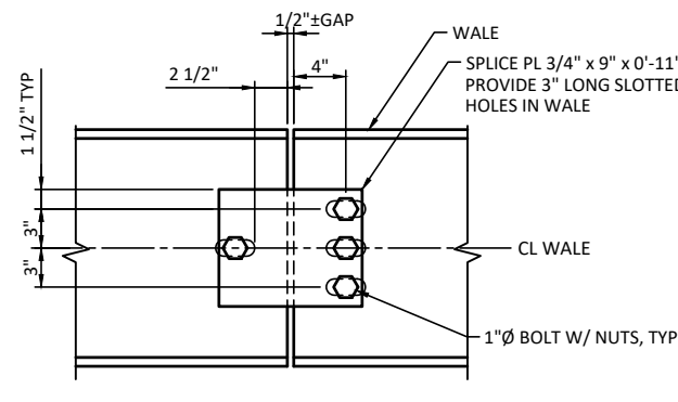
C DETAIL - WALE SPLICE FIG 1 SCALE: 1 1/2" = 1'-0"
