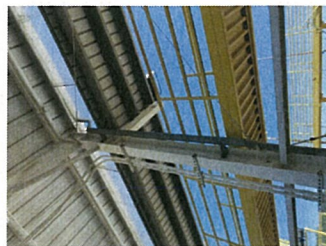
6 CANOPY FRAMING NTS A5.0
