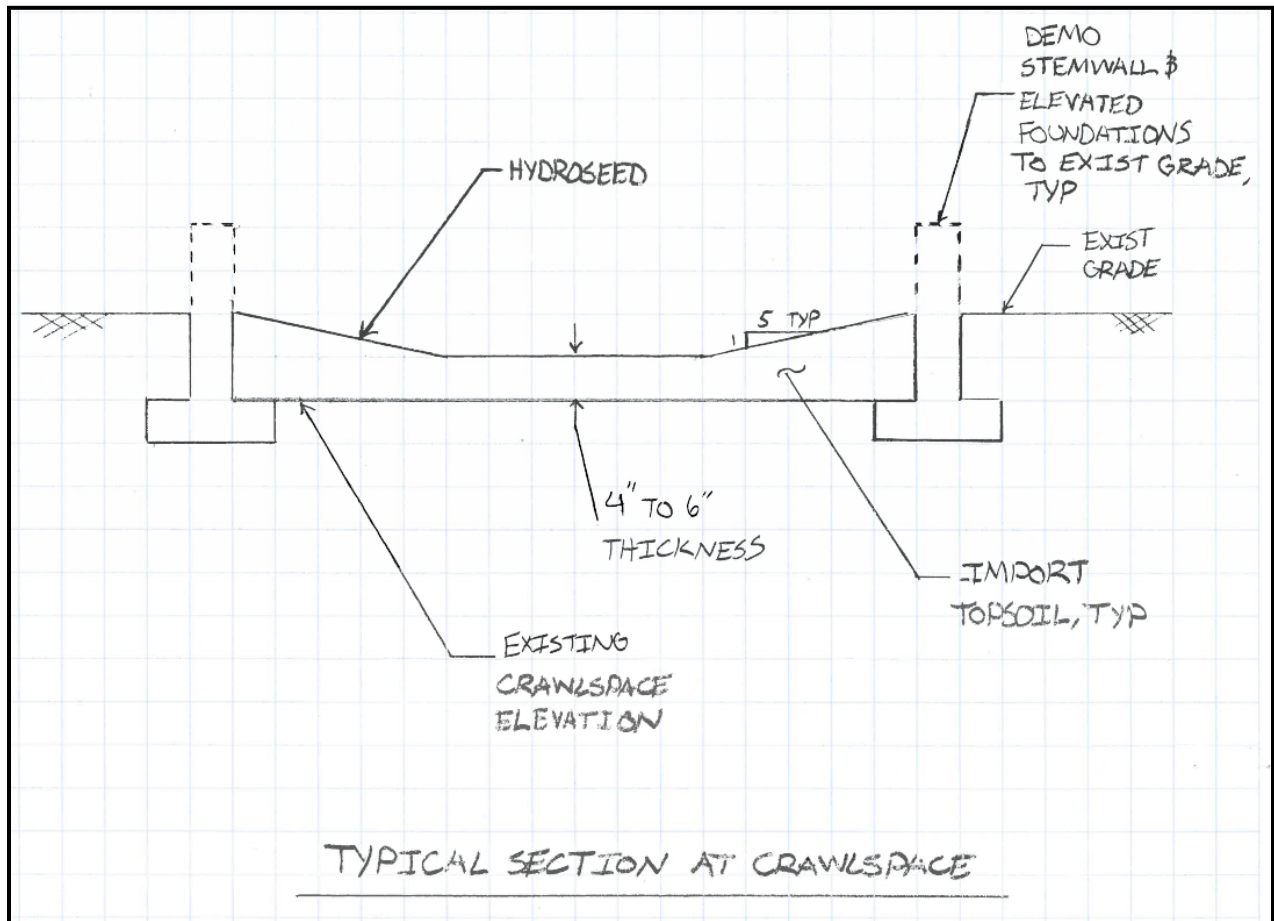
Figure 29 – 2338 E 11 th Street Typical Section at CrawlSpace
