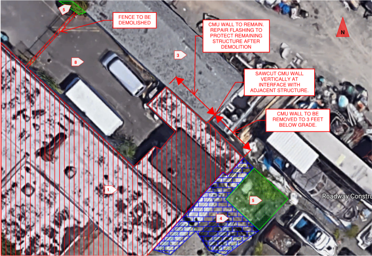
Figure 27 – 2338 E 11 th Street CMU Wall Demolition Plan View
