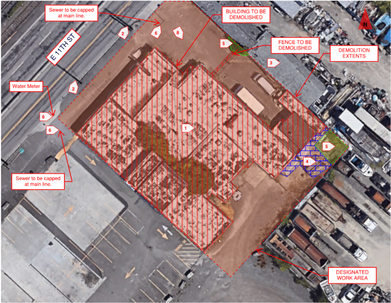
Figure 28 – 2338 E 11 th Street Building Demolition Plan View
