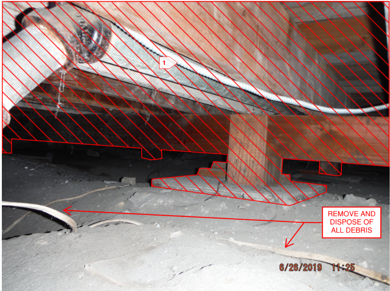
Figure 23 – 2338 E 11 th Street Building Demolition Interior Photograph
